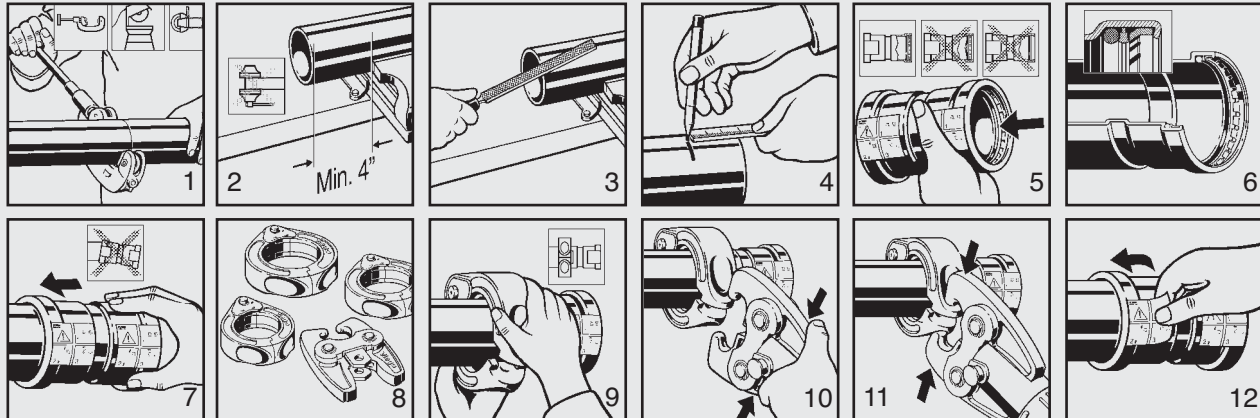
ProPress XL-C Insertion Depth Chart
